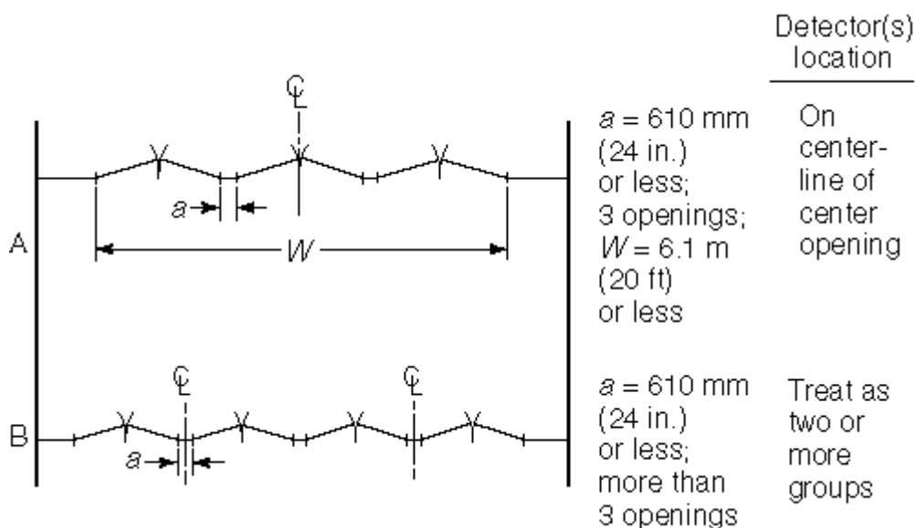
FIGURE 5.14.6.5.3.2 Detector Location Requirements for Group Doorways.
