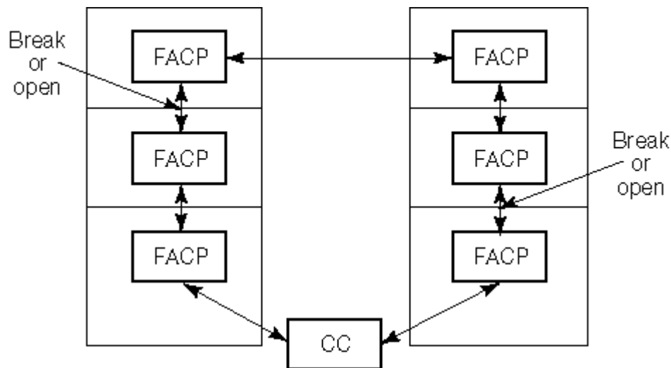
FIGURE C.3.14(h) Style 4 Fiber Network (Double Break).
