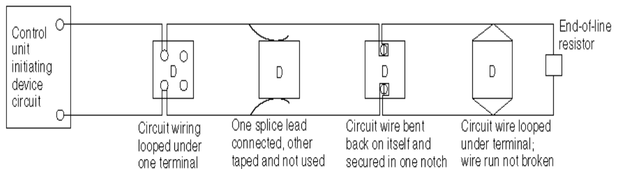
Incorrect wiring method — two-wire detectors
