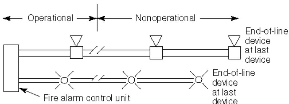
FIGURE C.2.12 Supervised Audible and Visible Notification Appliance Circuits.
