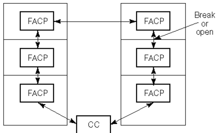
FIGURE C.3.14(i) Style 7 Fiber Network (Two LANs).
