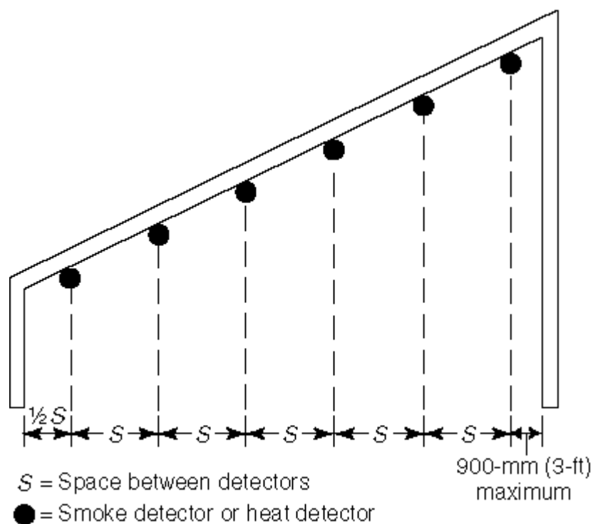
FIGURE A.5.6.5.4.2 Smoke or Heat Detector Spacing Layout, Sloped Ceilings (Shed
