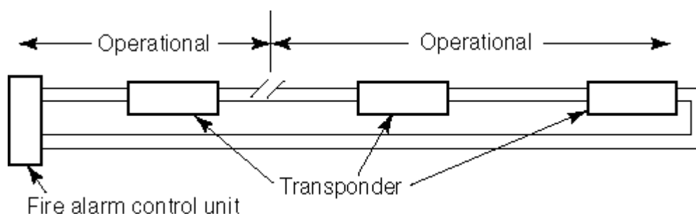
FIGURE C.3.12 Style 6.0 (Class A).
