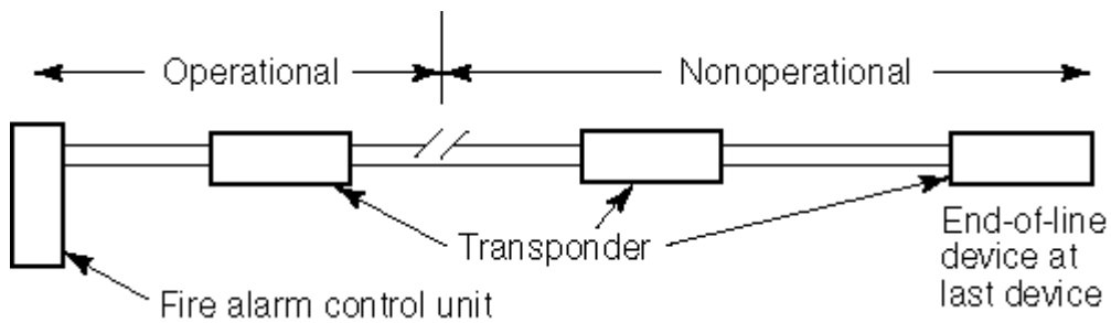
FIGURE C.3.9 Style 4.0 (Class B).
