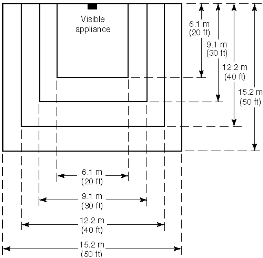
FIGURE 7.5.4.1.1 Room Spacing for Wall-Mounted Visible Appliances.
