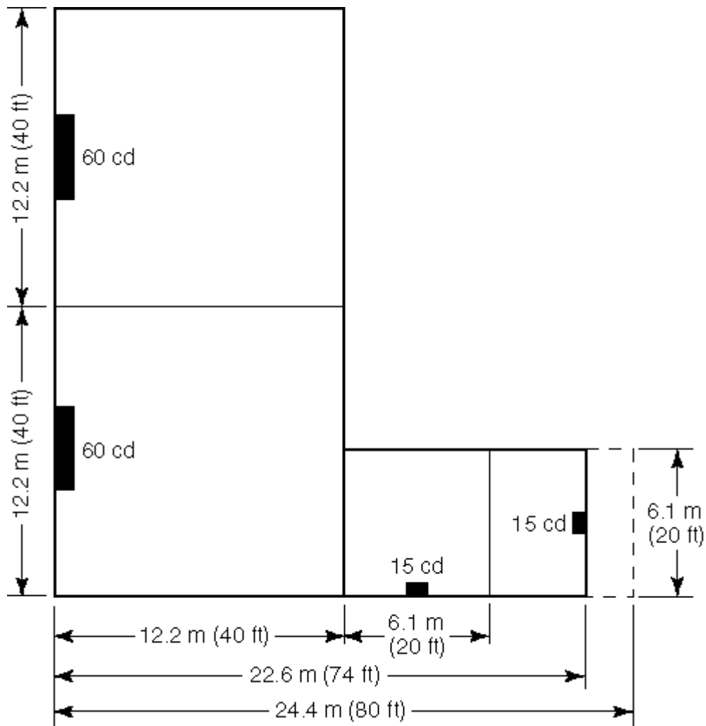
FIGURE A.7.5.4.1(b) Spacing of Wall-Mounted Visible Appliances in Rooms.
