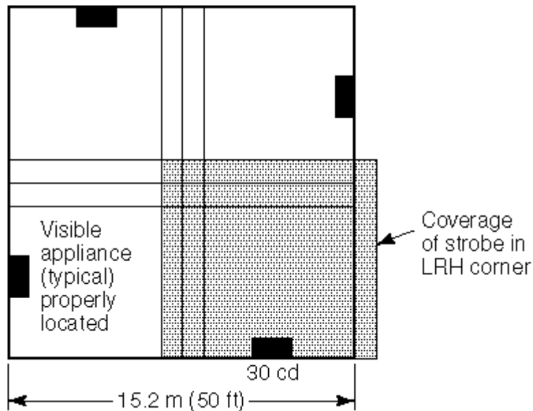
FIGURE A.7.5.4.1(c) Room Spacing Allocation — Correct.
