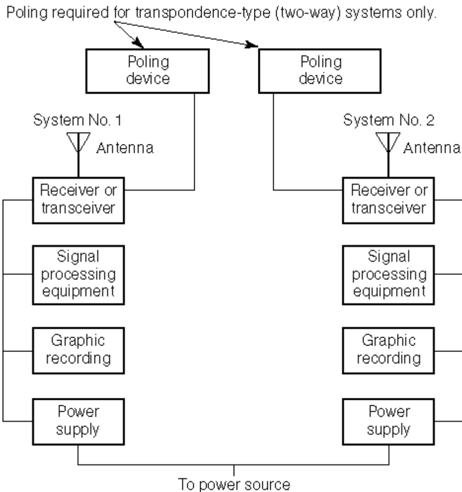
FIGURE A.9.5.3.1.1.1 Type A System Receiving Networks.
