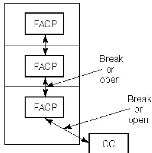
FIGURE C.3.14(g) Style 4 Fiber Network (Single Break).
