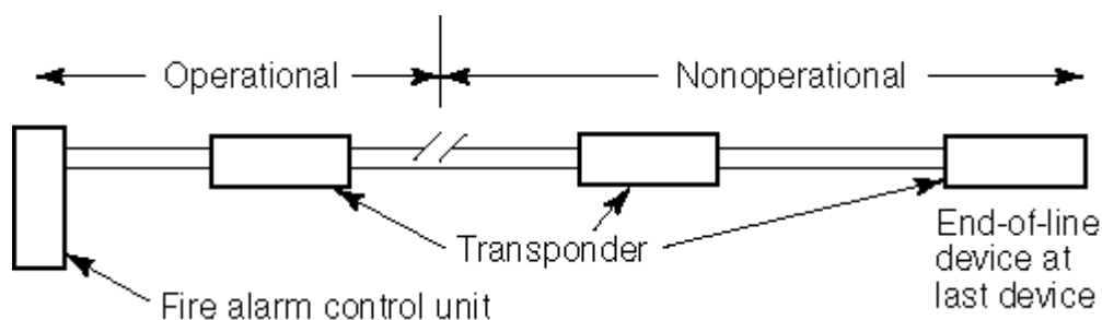
FIGURE C.3.7 Style 3.0 (Class B).
