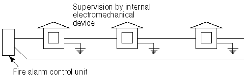
FIGURE C.3.4 Style 0.5(c) (Class B) Positive Supervised Successive.
