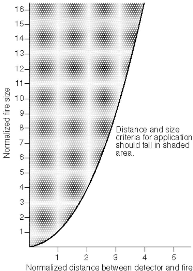
FIGURE A.5.8.3.1.1 Normalized Fire Size vs. Distance.
