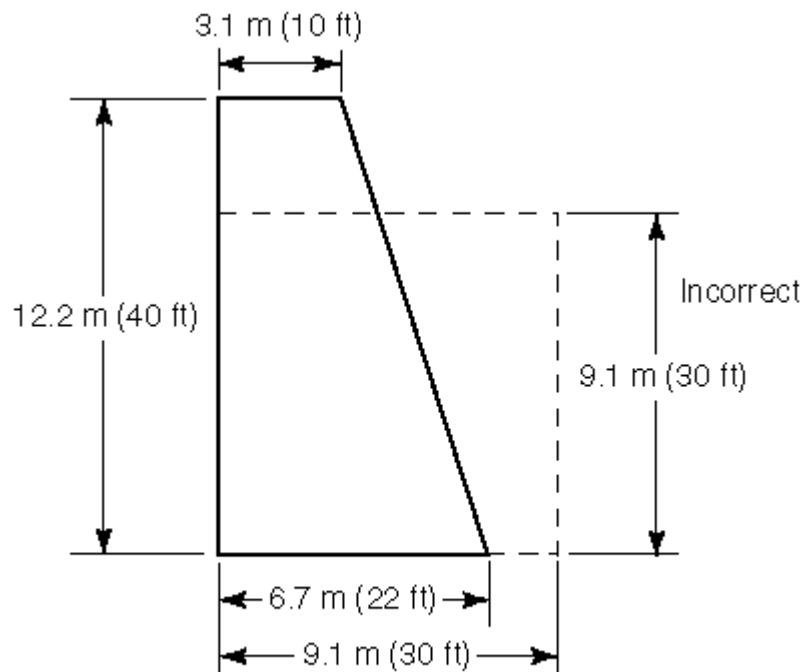
FIGURE A.7.5.4.1(a) Irregular Area Spacing.
