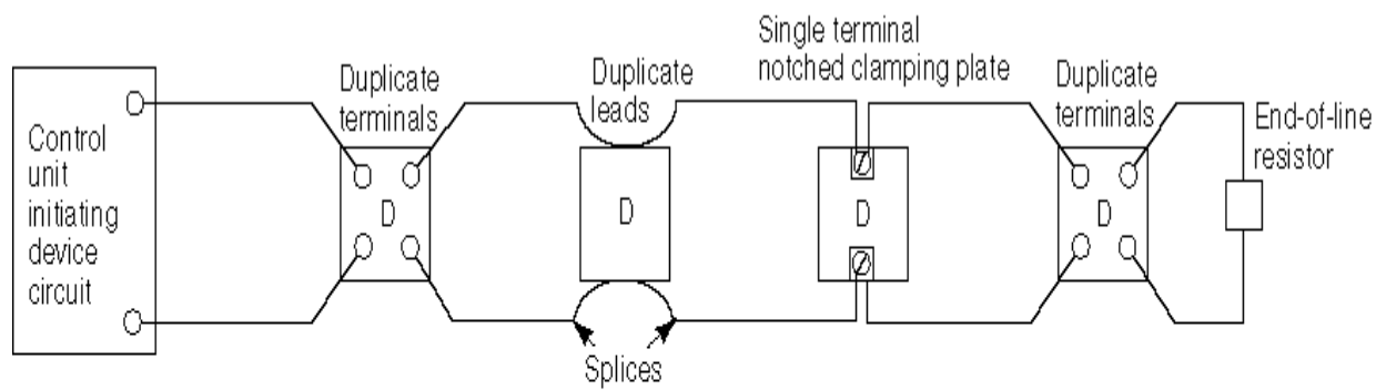
Correct wiring method — two-wire detectors
