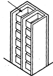
FIGURE 21.8.2.5(b) Tote Box Storeroom Showing Arrangement of Sprinklers and Baffles and Section of Tote Box Storage Rack. [42:Figure 6.7.7]
