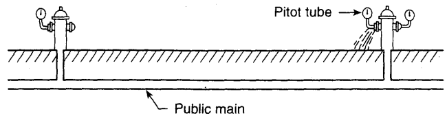
FIGURE A.23.2.1 Method of Conducting Flow Tests.
