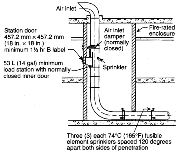
FIGURE A.21.16.2.1(g) Fire Damper Engineering Alternative for Penetration of Wall at Base of Shaft. [82:Figure A.5.3(e)]
