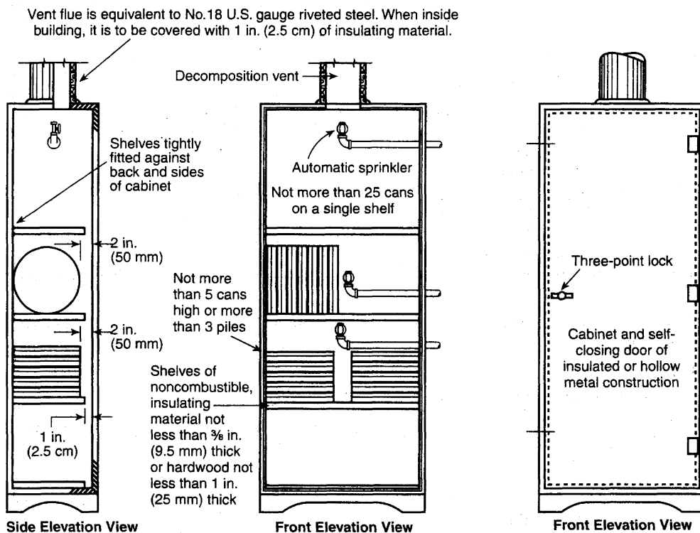
FIGURE 21.7.2.2.2 Standard Film Cabinet for Other Than Extended Term Storage Film. [40:Figure 6.2.1]
