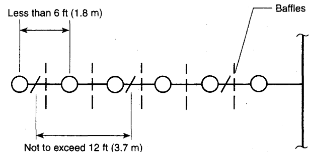
FIGURE A.9.2.3.2.2 Distance Between Hangers.
