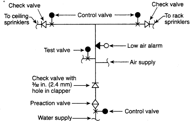
FIGURE 7.9.2.8.4 Valve Arrangement.
