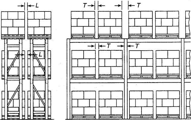
End View Double Row
