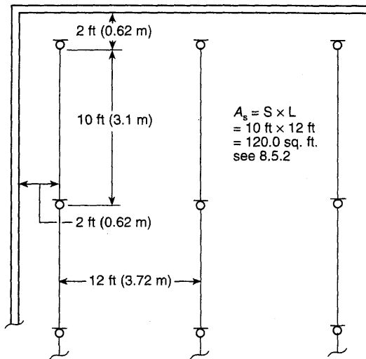
FIGURE A.22.4.4.5.3 Sprinkler Spacing.
