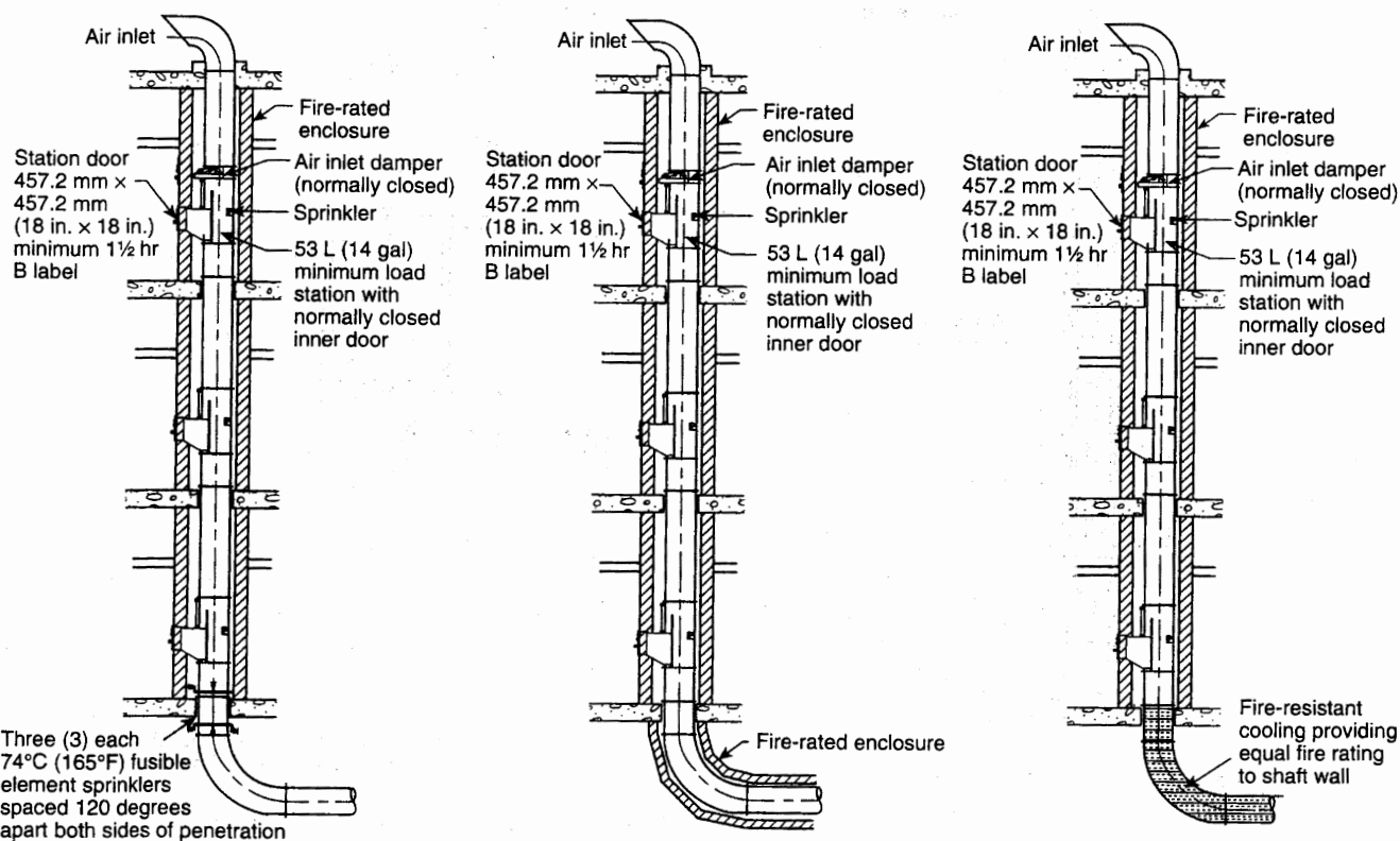
FIGURE A.21.16.2.1(d) Fire Damper Engineering Alternative for Penetration of Floor at Base of Shaft. [82:Figure A.5.3(b)]
