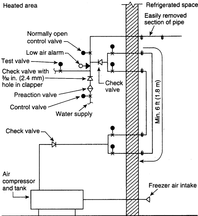
FIGURE 7.9.2.8.4 Valve Arrangement.
