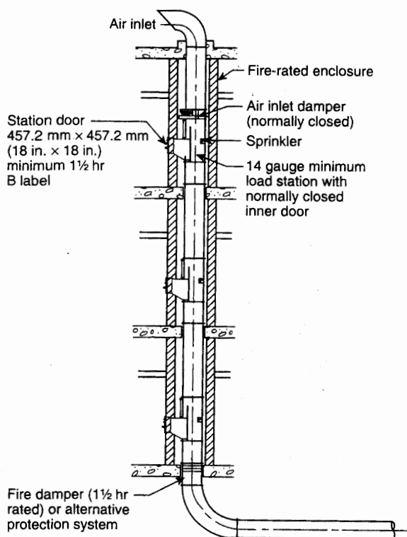
FIGURE A.21.16.2.1(c) Full Pneumatic System. [82:Figure A.5.3(a)]
