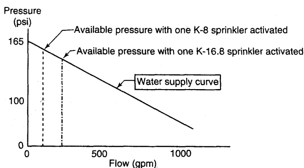
FIGURE A.12.6 Available Pressure Comparison.
