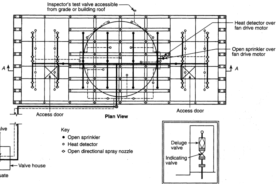
FIGURE A.21.24.2.3(a) Plan View, Typical Deluge Fire Protection Arrangement for Crossflow Towers with Completely Enclosed Distribution Basins. [214:Figure A.5.2.4.3(a)]
