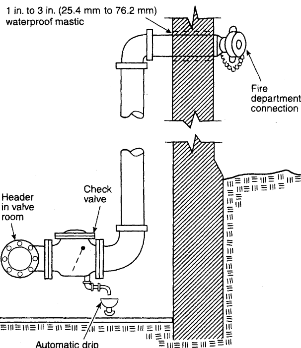
FIGURE 8.17.2.1 Fire Department Connections.
