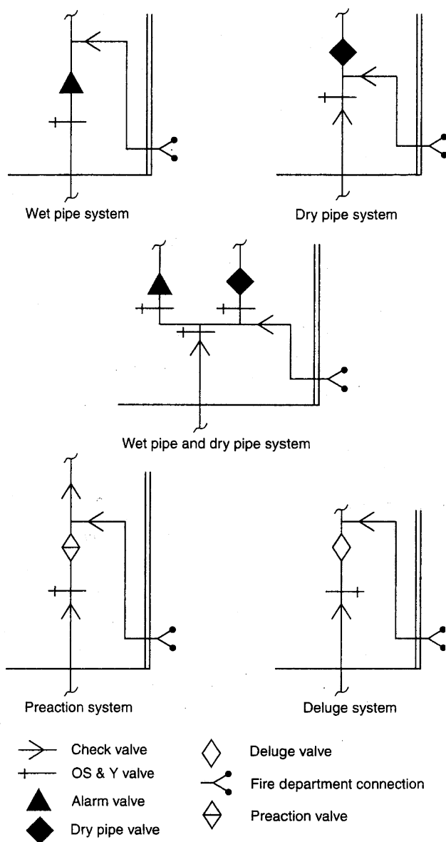
FIGURE A.8.16.1.1 Examples of Acceptable Valve Arrangements.
