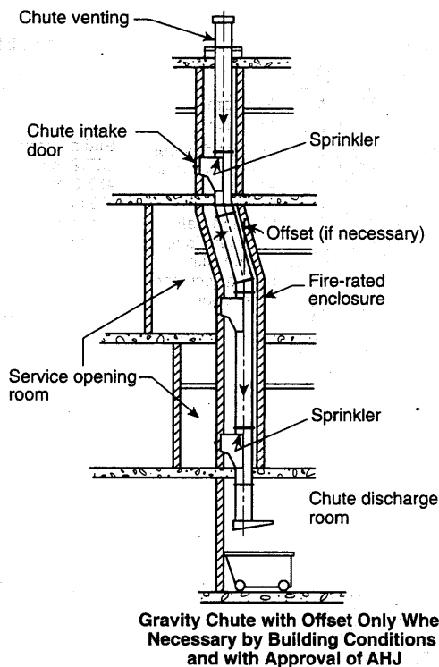
FIGURE A.21.16.2.1(b) Gravity Waste Chute. [82:Figure A.5.2(b)]
