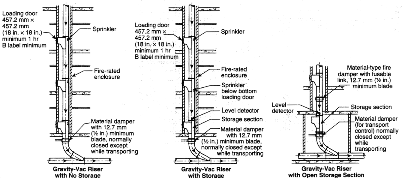
FIGURE A.21.16.2.1(h) Gravity Pneumatic System. [82:Figure A.5.4]
