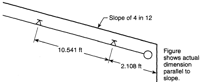
FIGURE A.22.4.4.5.6 Determination of Floor Area Under Sloped Ceiling/Roof.
