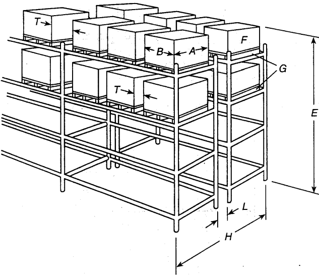
FIGURE A.3.9.3.7(a) Conventional Pallet Rack.
