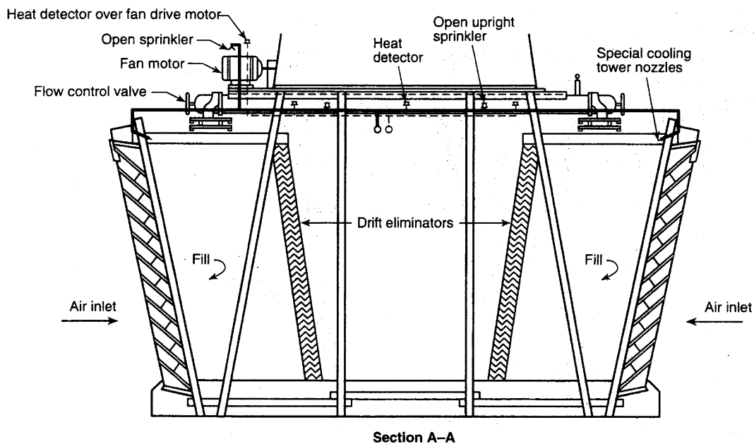
FIGURE A.21.24.2.2(d) Section View, Typical Deluge Fire Protection Arrangement for Multicell Crossflow Towers. [214:Figure A.5.2.4.2(d)]
