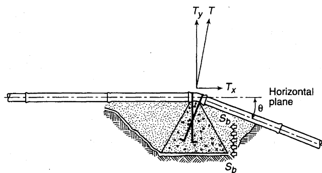
FIGURE A.10.8.2(b) Bearing Thrust Block. [24:Figure A.10.8.2(b)]
