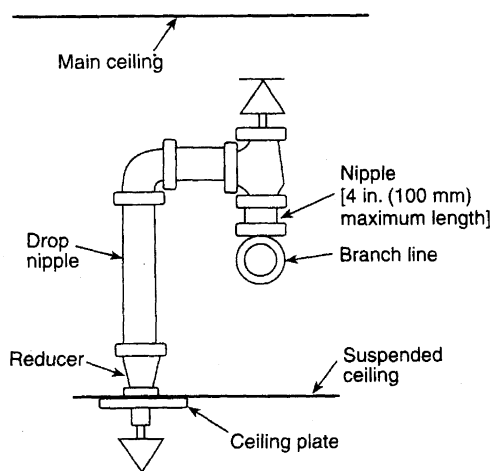
FIGURE 8.15.19.4.3 Sprinklers in Concealed Space and Below Ceiling.
