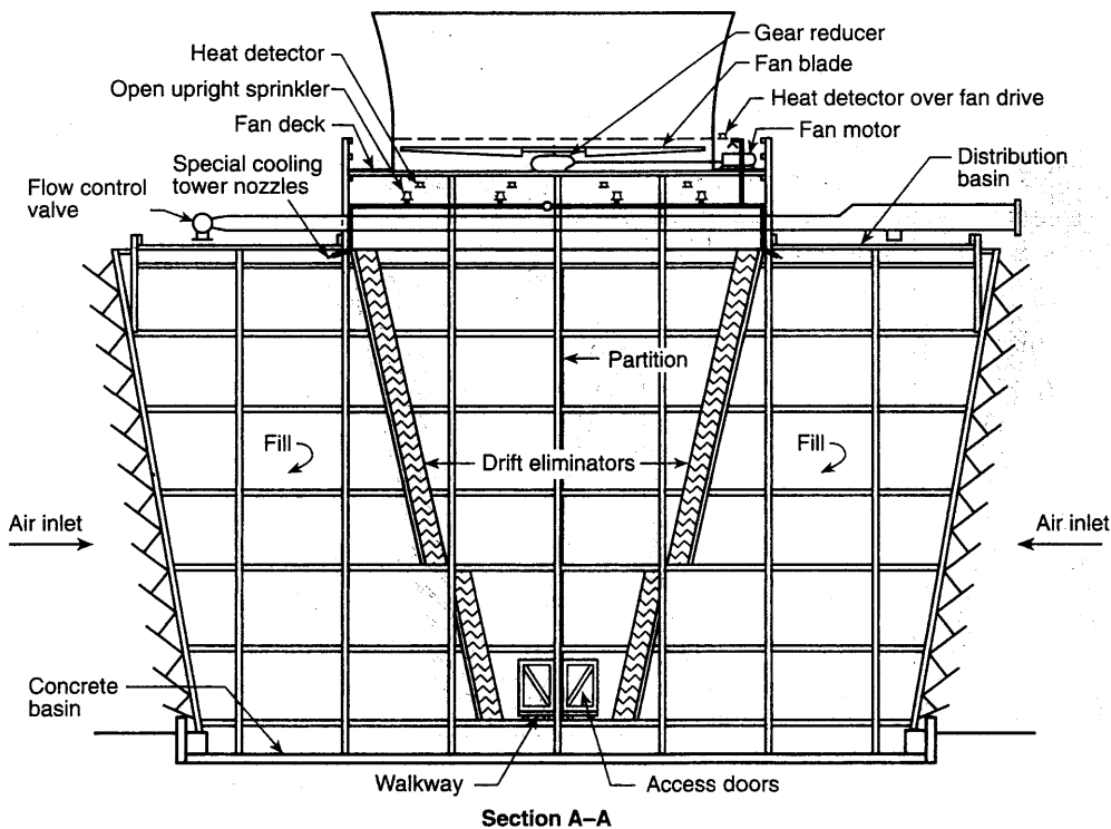
FIGURE A.21.24.2.2(b) Section View, Typical Deluge Fire Protection Arrangement for Crossflow Towers. [214:Figure A.5.2.4.2(b)]
