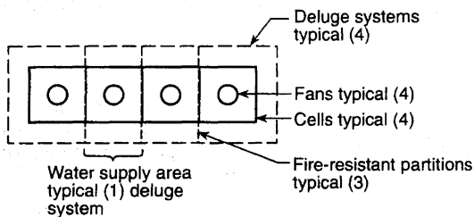
FIGURE A.21.24.1.7.1.3 Multiple Deluge Systems. [214:Figure A.5.6.1.3]
