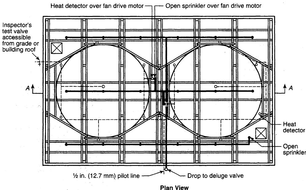
FIGURE A.21.24.2.1(a) Plan View, Typical Deluge Fire Protection Arrangement for Counter-flow Towers. [214:Figure A.5.2.4.1(a)]
