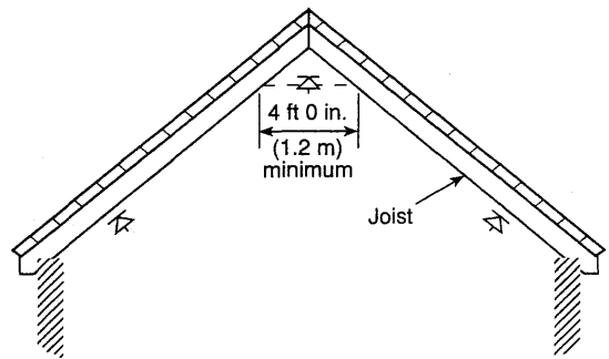
FIGURE 8.6.4.1.3.3 Horizontal Clearance for Sprinklers at Peak of Pitched Roof.
