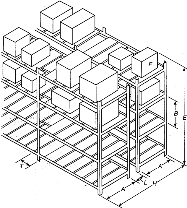
FIGURE A.3.9.3.7(c) Double-Row Racks with Solid Shelves.
