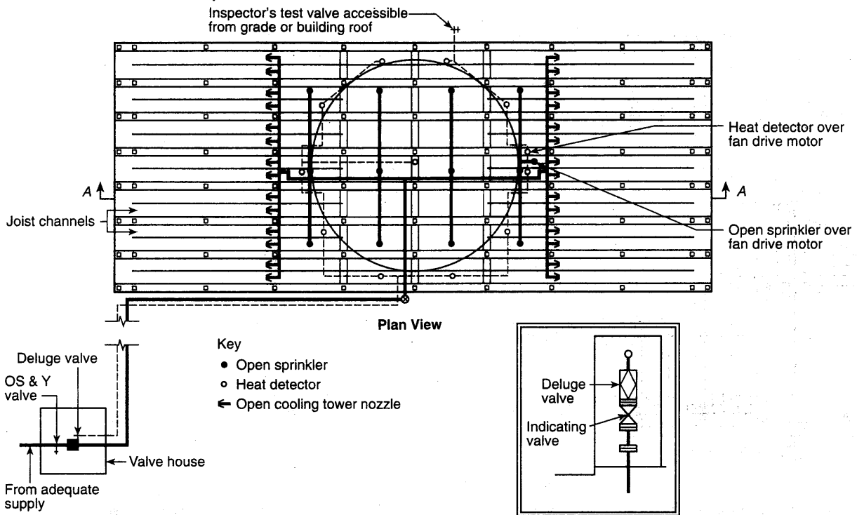
FIGURE A.21.24.2.2(a) Plan View, Typical Deluge Fire Protection Arrangement for Crossflow Towers. [214:Figure A.5.2.4.2(a)]
