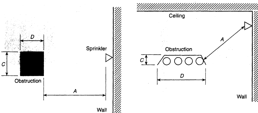
Plan View of Column
