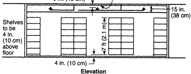
FIGURE 21.8.2.5(a) Tote Box Storeroom Showing General Arrangement of Racks and Sprinklers. [42:Figure 6.7]
