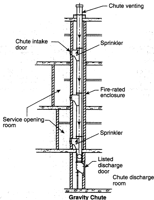
FIGURE A.21.16.2.1(a) Gravity Linen Chute. [82:Figure A.5.2(a)]
