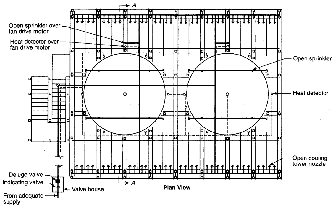
FIGURE A.21.24.2.2(c) Plan View, Typical Deluge Fire Protection Arrangement for Multicell Crossflow Towers. [214:Figure A.5.2.4.2(c)]
