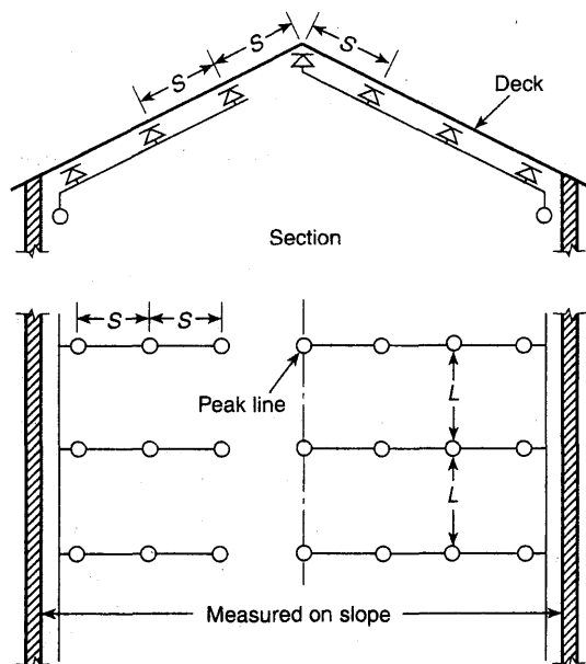
FIGURE 8.10.3.4(a) Maximum Distance Between Sprinklers with Sloped Ceilings — Arrangement A.
