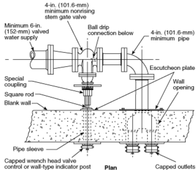
Figure A-4-2.2 Typical wall fire hydrant installation
