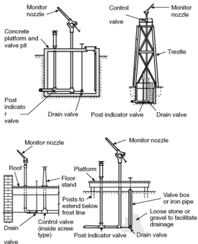
Figure A-6-1(b) Typical hydrant-mounted monitor nozzle
