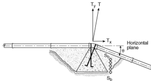
Figure A-8-6.2.1(b) Gravity thrust block
