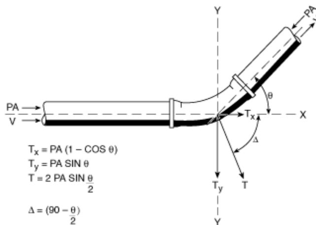
Figure A-8-6.2(b) Typical connection to a fire protection system riser
