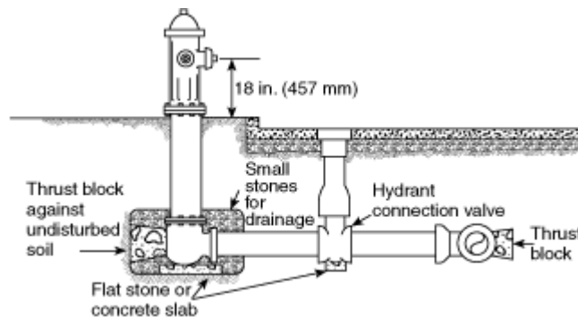
Figure A-4-3.3 Typical hydrant connection
